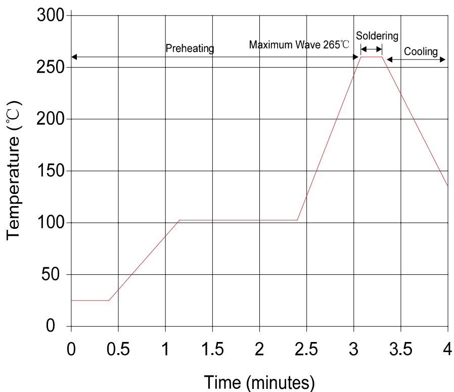
Wave Lead Free Soldering Recommendation
