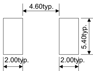
Recommended Pad Layout (mm)
