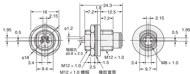
XS3P-M421-2 (焊帽端子)
