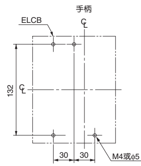
带外部操作手柄(V, N)
