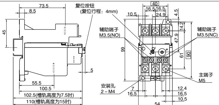
TR-N2H/3型, TR-N2HQ型 TK-N2H/3型, TK-N2HQ型
