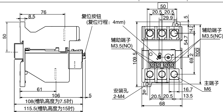
TR-N3H/3型, TR-N3HQ型 TK-N3H/3型, TK-N3HQ型
