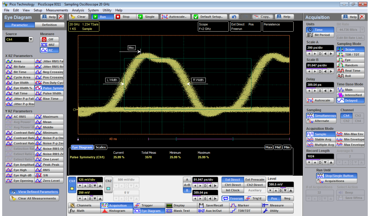
RZ Pulse Symmetry definition
