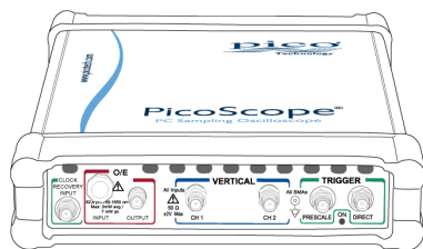
The PicoScope 9321 Dual-channel 20 GHz electrical Sampling Oscilloscope with 9.5 GHz optical to electrical converter and 11.3 Gb/s clock recovery
