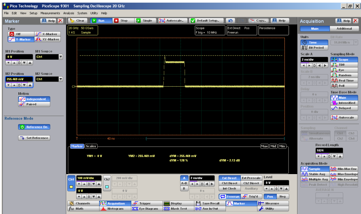
Ratiometric measurement of Overshoot with Y Markers
