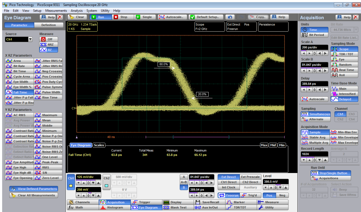
RZ Fall Time definition
