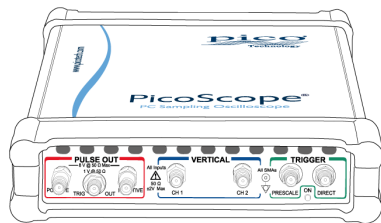
The PicoScope 9311 Dual-channel 20 GHz Sampling Oscilloscope with 60 ps 6 V differential TDR/TDT
