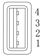
USB/A(公)(前视图)
