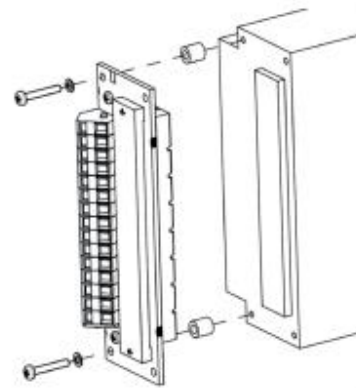
Fig. 34 Cage clamp adapter HZZ00144-G
