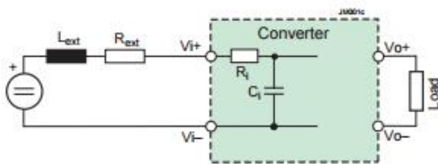
Fig. 6 Equivalent input circuit
