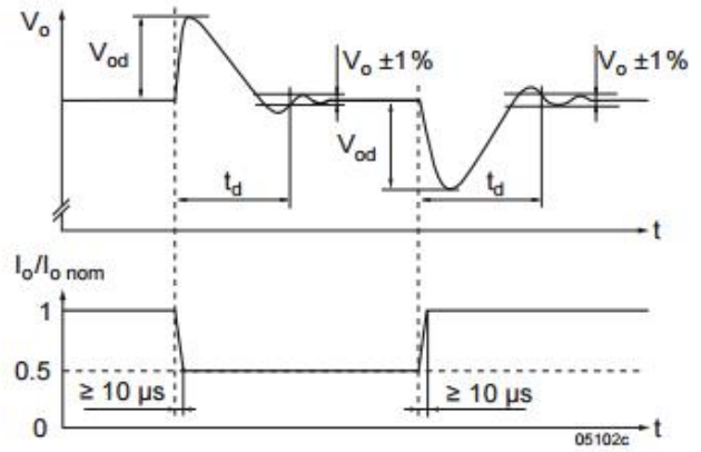
Fig. 13 Typical dynamic load regulation of V_o
