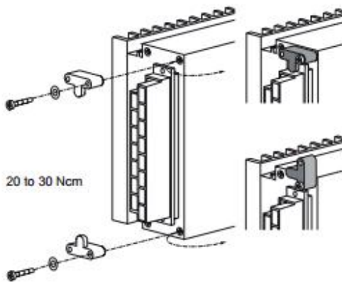
Fig. 33 Connector retention brackets HZZ01216-G
